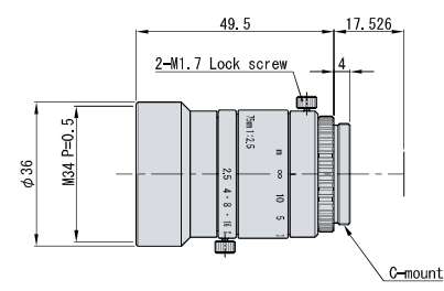
CVL-7525M
