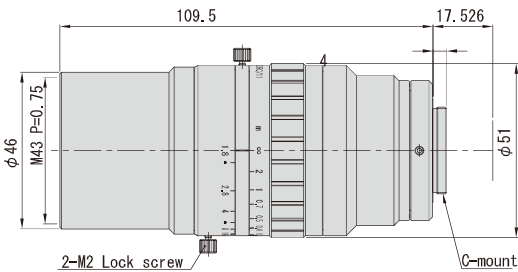
CVL-2518-IR11
