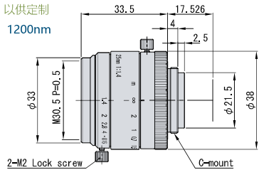
CVL-2514M1-IR1200
