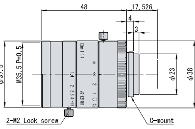
CVL-1214M1
