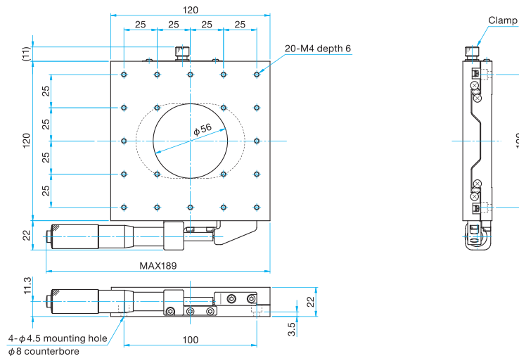
MLT31-120SRH Hexagonal socket head cap screw M4x8...4 screws
