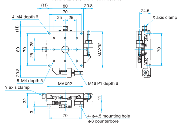
MLT32-80SDM Hexagonal socket head cap screw M4x8...4 screws
