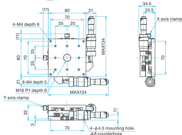
MLT32-80SDM Hexagonal socket head cap screw M4x8...4 screws
