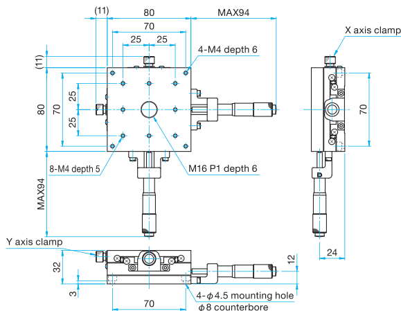
MLT32-80S Hexagonal socket head cap screw M4x8...4 screws
