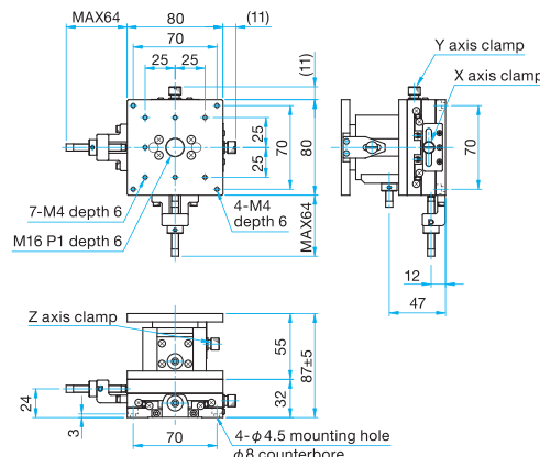
MLT35-80SFP Hexagon socket head cap screw M4×8...4 screws 3mm
