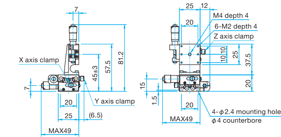
MLT35-25SL Pan head screw M2x4...4 screws
