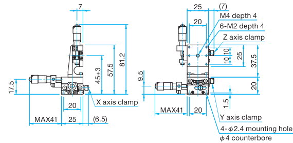
MLT35-25CL Pan head screw M2x4...4 screws
