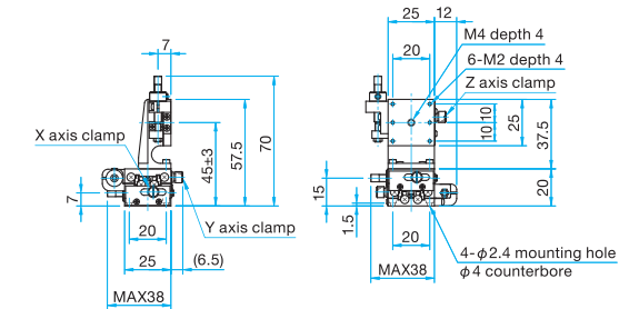
MLT35-25SLFP Pan head screw M2x4...4 screws 2mm
