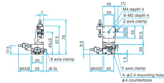
MLT35-25CLFP Pan head screw M2x4...4 screws 2mm
