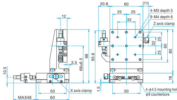
MLT34-60CLFP Hexagonal socket head cap screw M4x6...4 screws 3mm
