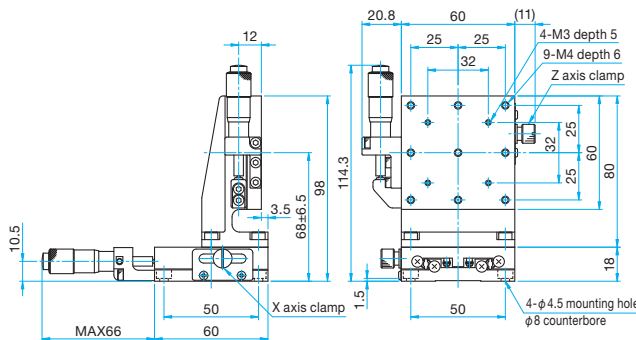
MLT34-60CL Hexagonal socket head cap screw M4x6...4 screws
