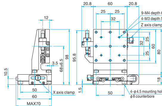
MLT34-60SLFP Hexagonal socket head cap screw M4x6...4 screws 3mm
