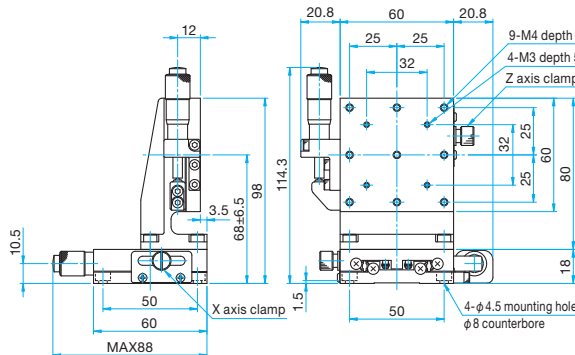
MLT34-60SL Hexagonal socket head cap screw M4x6...4 screws
