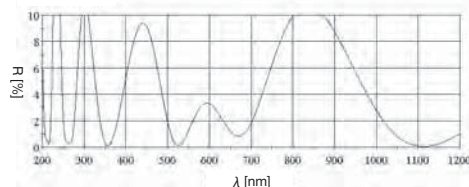
Notch filter
