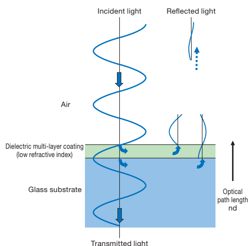
Image of single-layer dielectric Anti-reflection coating structure
