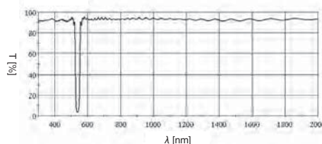
Notch filter
