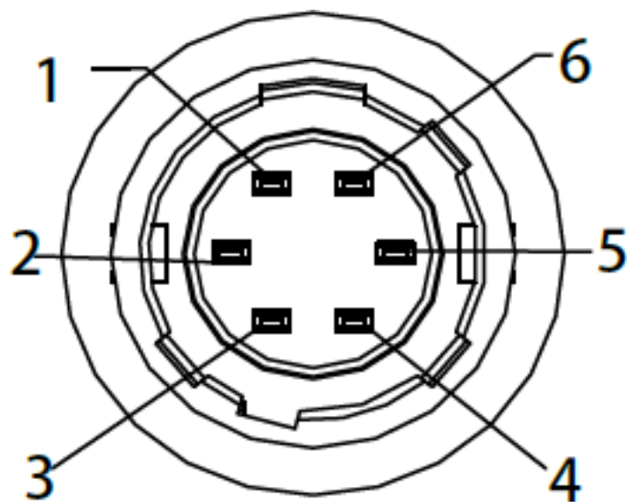
Fig. 32: Pin Numbering for the 6-pin Connector
