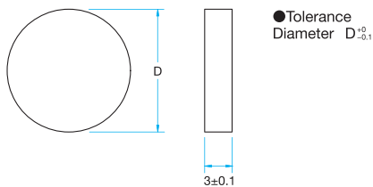
Outline Drawing
