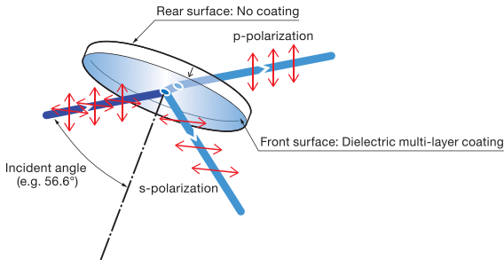
Schematic
