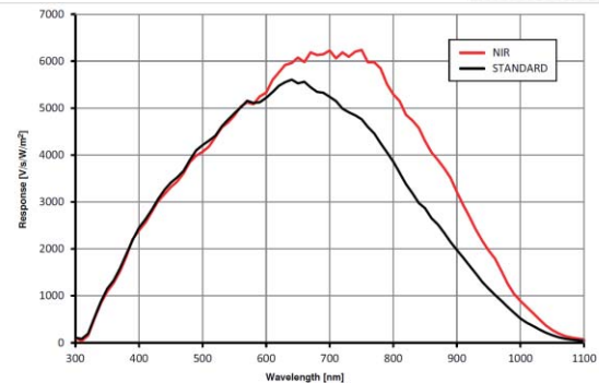
CHGM-530N Quantum Efficiency
