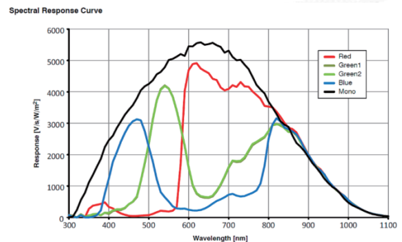
CHGM-530M/C-1 Quantum Efficiency
