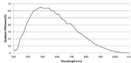
CHGM-503M-14 Quantum Efficiency
