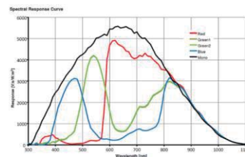
CHGM-230C Quantum Efficiency
