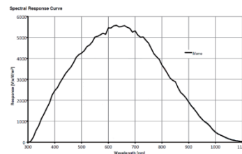
CHGM-230M Quantum Efficiency
