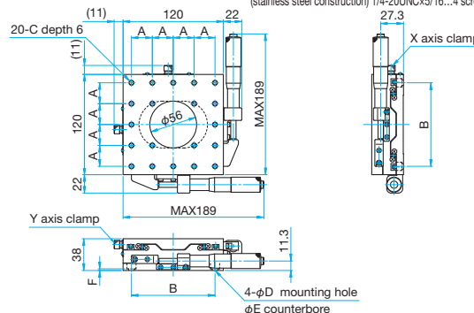
TSD-1202SH-M6/1202SHUU Hexagonal socket head cap screw M6x8...4 screws (M6) Hexagonal socket head cap screw (stainless steel construction) 1/4-20UNCx5/16...4 screws (UU)
