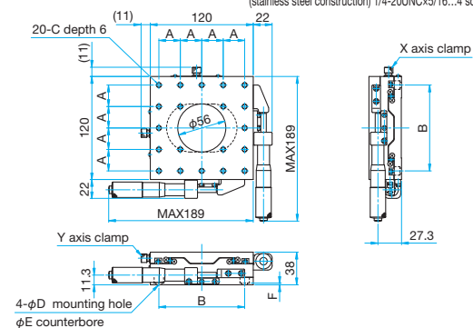
TSD-1202SRH-M6/1202SRHUU Hexagonal socket head cap screw M6x8...4 screws (M6) Hexagonal socket head cap screw (stainless steel construction) 1/4-20UNCx5/16...4 screws (UU)
