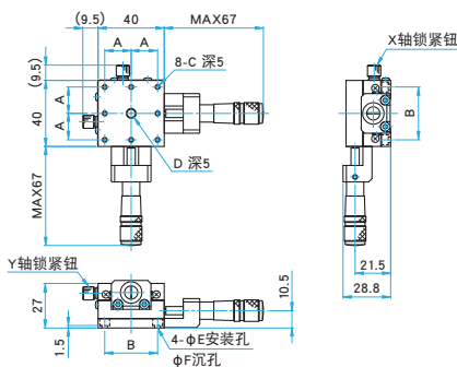
TSDS-402C/402CUU
