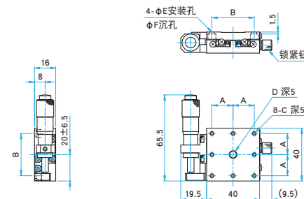
TSD-401SRZ/401SRZUU
