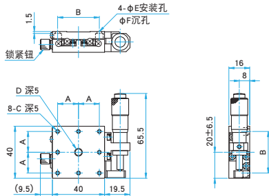
TSD-401SZ/401SZUU
