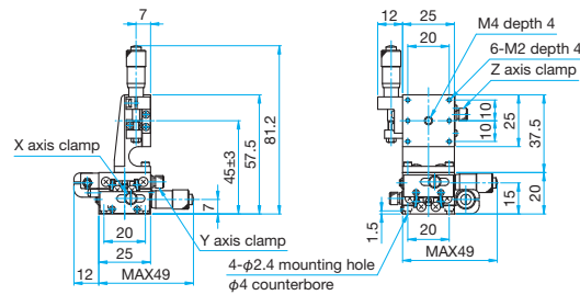
TSD-255SRL Hexagonal socket head cap screw M2x4...4 screws
