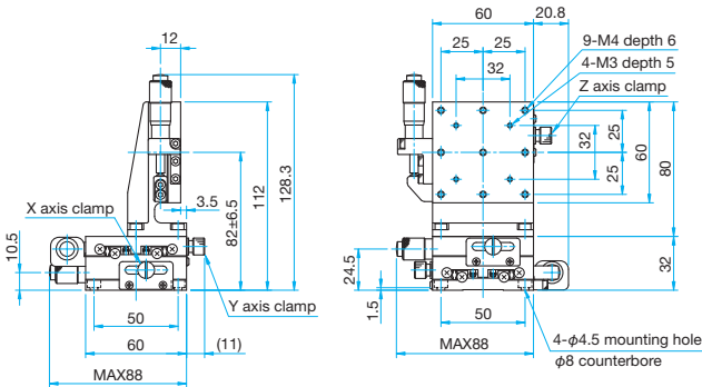
TSD-655CL-M6/655CLUU Hexagonal socket head cap screw M6x6...4 screws (M6) Hexagonal socket head cap screw 1/4-20UNCx1/4...4 screws (UU)
