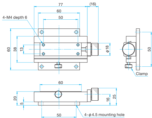
MLT11-2060 Hexagonal socket head cap screw M4x10...4 screws
