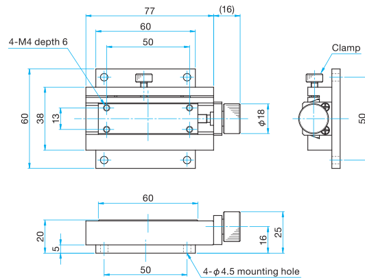
MLT11-2060R Hexagonal socket head cap screw M4x10...4 screws
