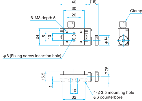
MLT11-2430R Pan head screw M3x5...4 screws
