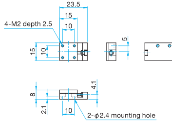
MLT11-15 Pan head screw M2x4...2 screws 2.5mm
