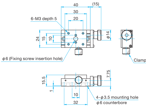
MLT11-2430 Pan head screw M3x5...4 screws
