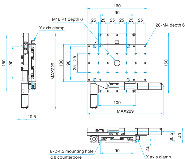
MLT32-1016S Hexagonal socket head cap screw M4x8...4 screws
