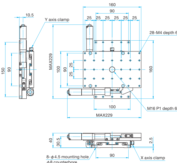
MLT32-1016SR Hexagonal socket head cap screw M4x8...4 screws
