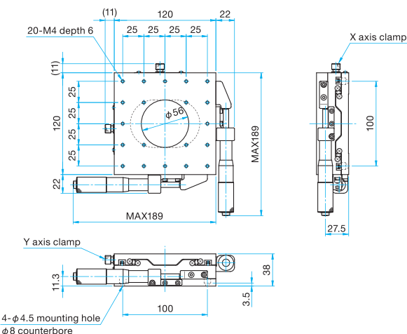
MLT32-120SRH Hexagonal socket head cap screw M4x8...4 screws
