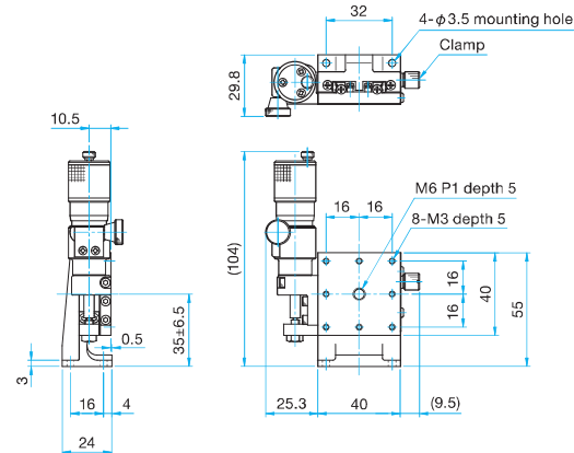
MLT33-40LWP Hexagon socket head cap screw M3×6...4 screws
