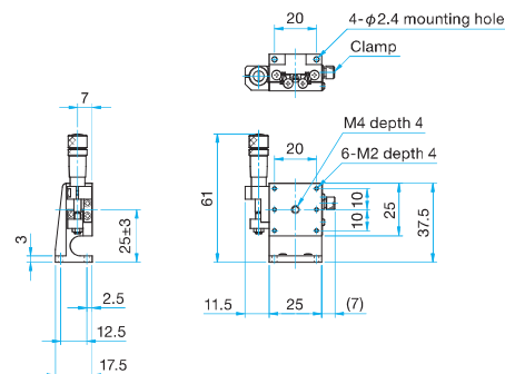
MLT63-25L Hexagon socket head cap screw (stainless steel construction) M2×6...4 screws
