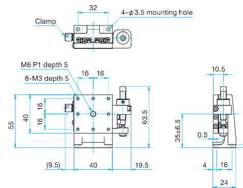
MLT33-40RLFP Hexagon socket head cap screw M3×6...4 screws 3mm
