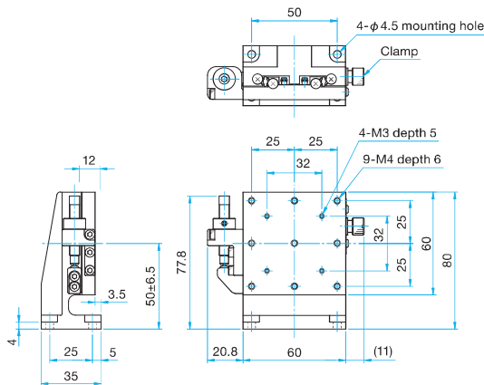
MLT33-60LFP Hexagonal socket head cap screw M4x8...4 screws 3mm
