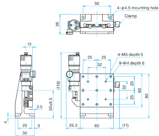
MLT33-60LWP Hexagonal socket head cap screw M4x8...4 screws
