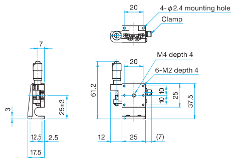
MLT33-25L Hexagonal socket head cap screw M2×6...4 screws
