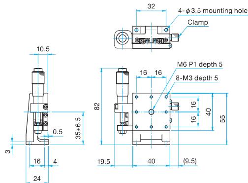
MLT33-40L Hexagon socket head cap screw M3×6...4 screws
