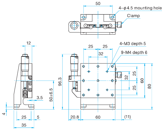
MLT33-60L Hexagonal socket head cap screw M4x8...4 screws
