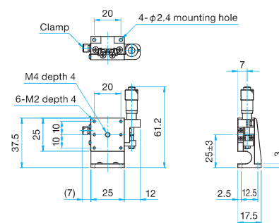
MLT33-25RL Hexagonal socket head cap screw M2×6...4 screws
