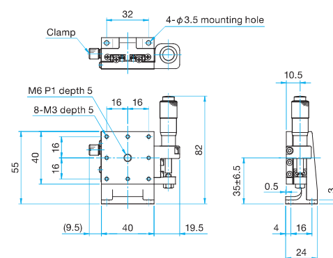
MLT33-40RL Hexagon socket head cap screw M3×6...4 screws
