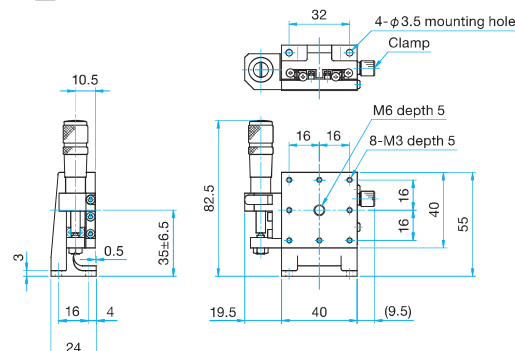
MLT63-40L Hexagon socket head cap screw (stainless steel construction) M3×6...4 screws
