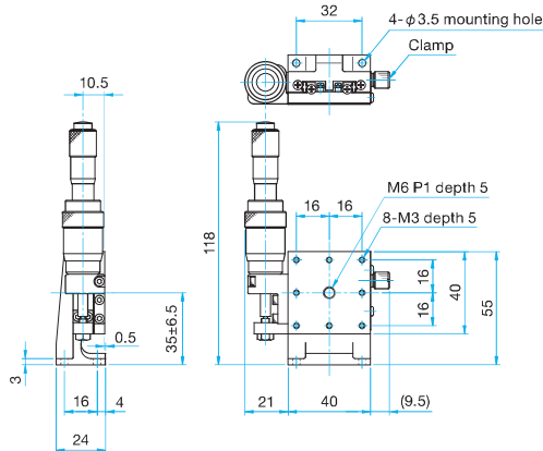
MLT33-40DML Hexagon socket head cap screw M3×6...4 screws
