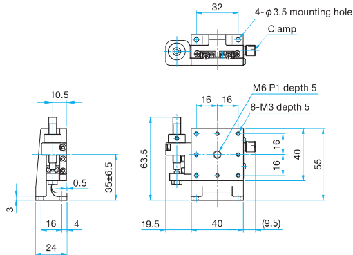
MLT33-40LFP Hexagon socket head cap screw M3×6...4 screws 3mm
