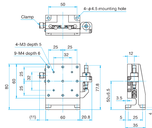
MLT33-60RLFP Hexagonal socket head cap screw M4x8...4 screws 3mm
