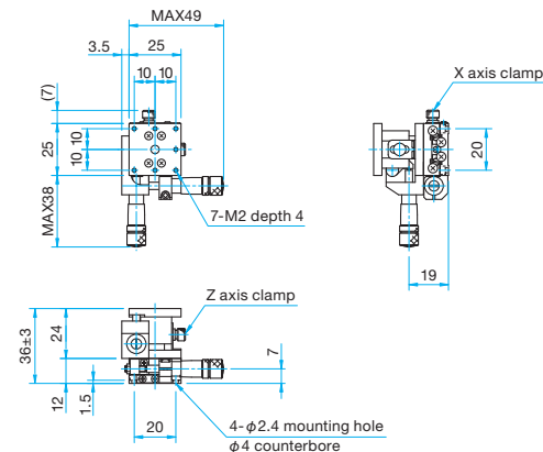
MLT64-25S Hexagon socket head cap screw (stainless steel construction) M2x4...4 screws
